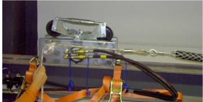
BKS 400 used as capstan winch in a tray
